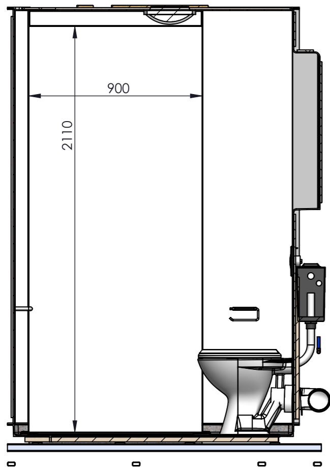
SECTION L-L
